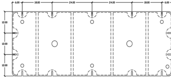
MOUNTING SLOT DETAIL SCALE 2:1 ALL DIMS NOMINAL
