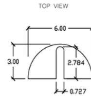
MOUNTING SLOT DETAIL SCALE 2:1 ALL DIMS NOMINAL
