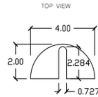
MOUNTING SLOT DETAIL SCALE 2:1 ALL DIMS NOMINAL
